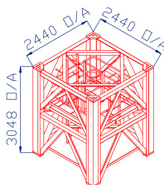
TOWER TYPE 1150
