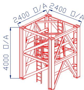
TOWER TYPE 392
