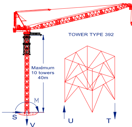
CRANE FREE-STANDING WITH EXTERNAL CLIMBER
