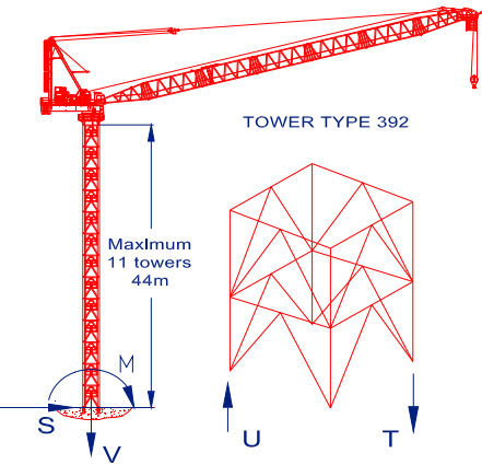
CRANE FREE-STANDING WITHOUT EXTERNAL CLIMBER
