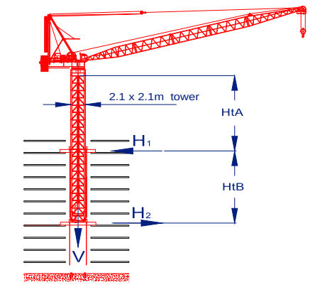
INTERNAL CLIMBER ON COLLARS
