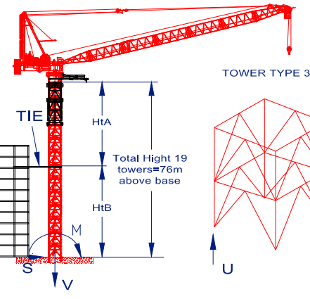
WITH CLIMBER- ONE TIE ABOVE THE BASE
